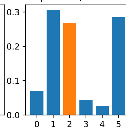
pred. -1, true 2
