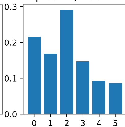
pred. -1, true -1
