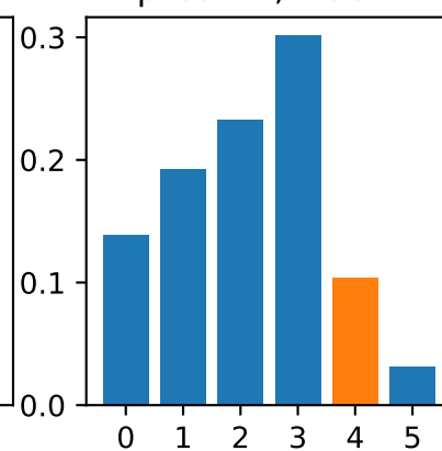
pred. -1, true 4
