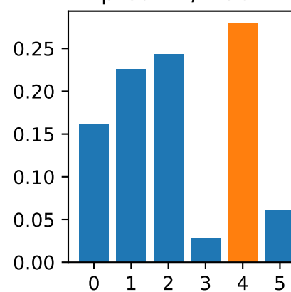
pred. -1, true 4
